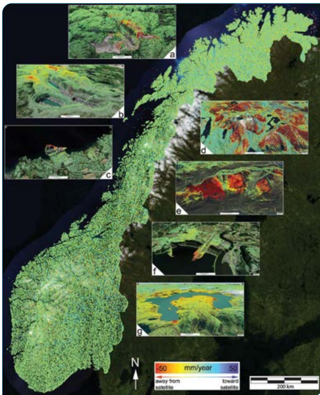
Fig. 2 InSAR Norway: nationwide ground deformation mapping and selected application examples: (a) settlement in mine tailings, (b) instabilities in the open-pit Bjørnevatn mine in Finnmark, (c) subsidence in reclaimed land at Grillstadjæra in Trondheim, (d) permafrost-related ground deformation, (e) unstable slopes at Piggstind and Sjøvasstind in Troms, (f) subsidence in reclaimed land at Trondheim Airport, Værnes, and (g) deformation affecting the Storglomvatn hydropower dam. [Attribution: Gökhan Aslan (InSAR Norway, NGU)]
