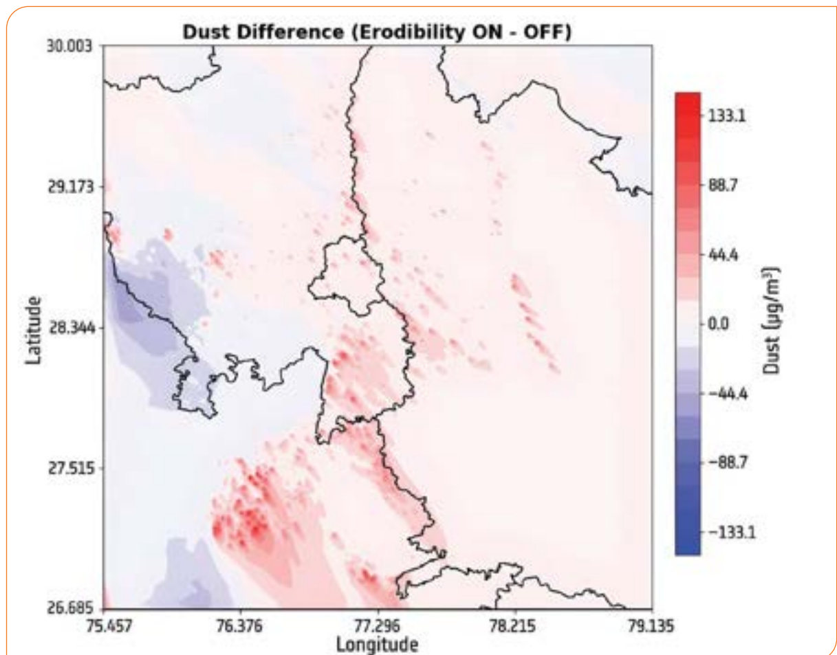
Fig. 5 Spatial distribution of the dust concentration ( \mu\text{g}/\text{m}^3 ), originating from identified barren land in Delhi-NCR on 28 th March 2025
