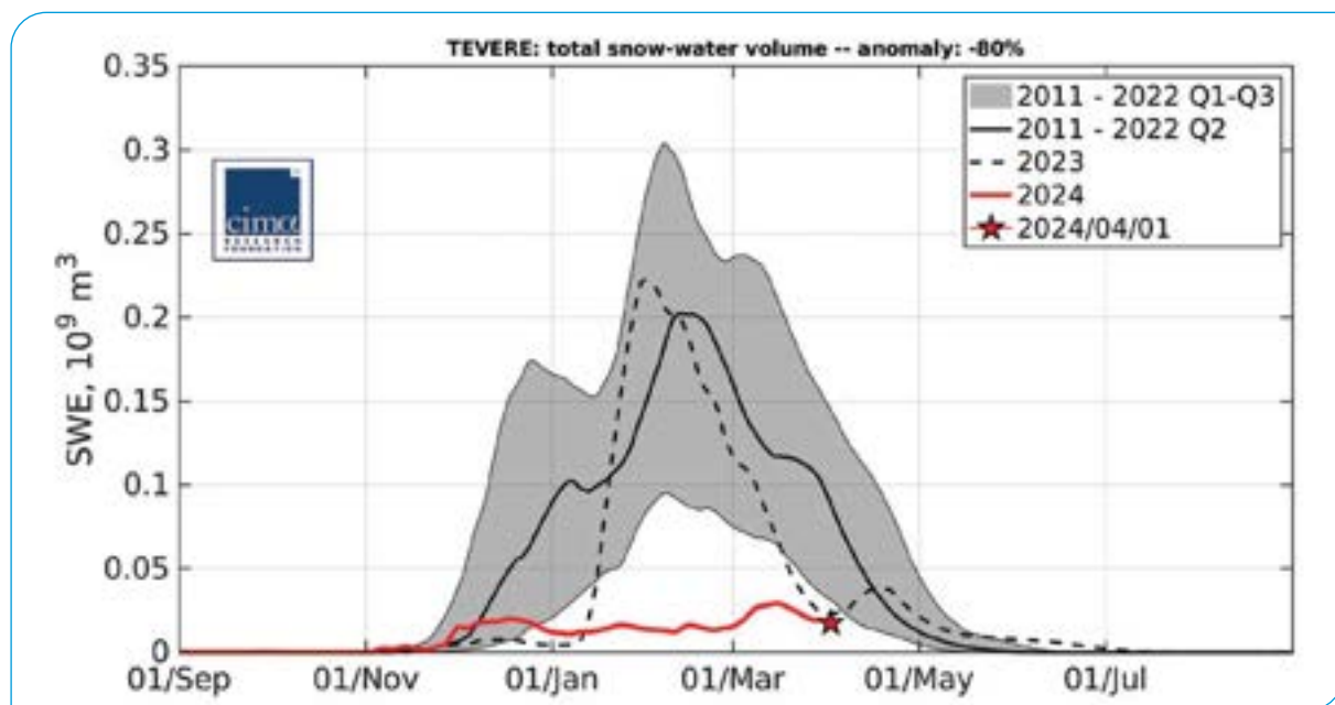
Fig. 2 Seasonal evolution of total SWE for the Tiber basin in real-time, during the season 2023-24 (red) as opposed to the long-term median (black line) and the 2022-23 season (dashed black line)
