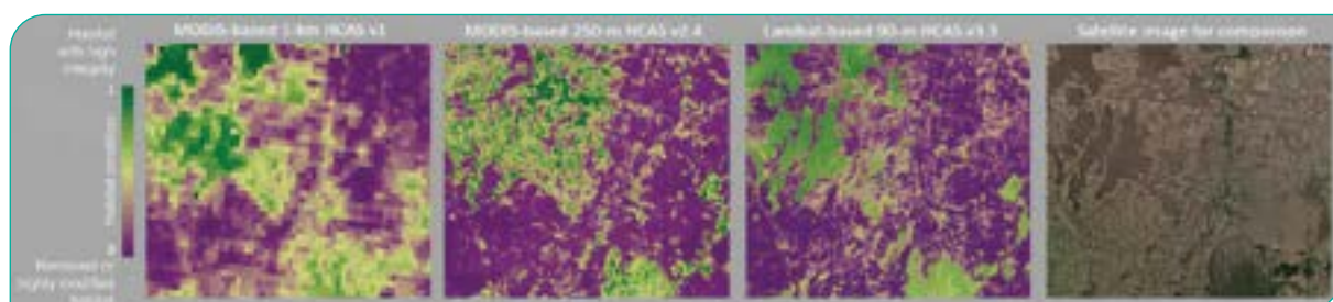
Fig. 3 Evolution of HCAS (Attribution: CSIRO, Landsat imagery courtesy of the U.S. Geological Survey, processed via Google Earth Engine)
