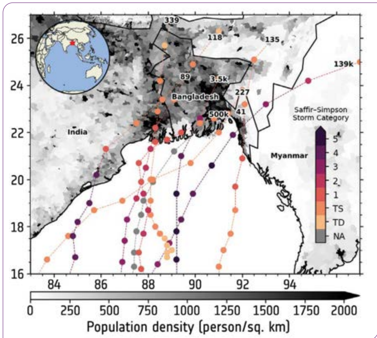
Fig. 1 Trajectories and intensities of major cyclones that have struck the Bengal Delta over the past five decades, with the number of victims recorded for each [Attribution: © Jamal Uddin Khan (LIENSs, La Rochelle)]
