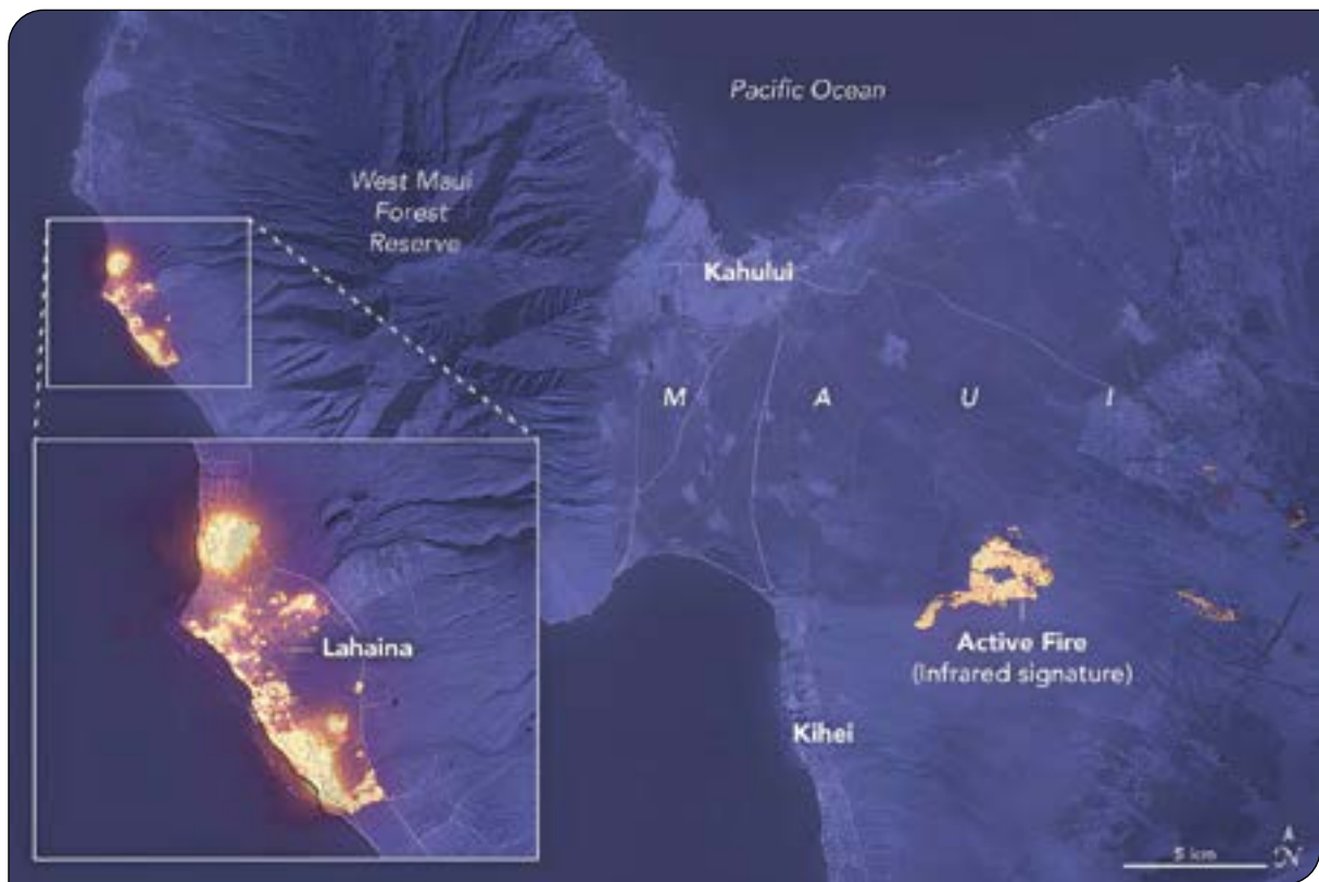
Fig. 5 Shortwave infrared imagery of wildfires burning in Lahaina and northeast of Kihei, Maui on Aug. 8, 2023. Fires are shown in yellow (Attribution: NASA Earth Observatory image by Lauren Dauphin, using Landsat data from the U.S. Geological Survey)
