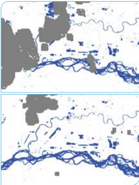
Fig. 2 Surface water extent over Fairbanks, Alaska. Image 2a is June 16 th , 2024, and Image 2b is June 17 th , 2024 (Attribution: JPL/OPERA)
