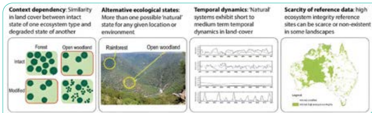
Fig. 2 The four main types of ecological application challenges for satellite remote sensing (Attribution: Harwood et al. (2016); Williams et al. (2024))
