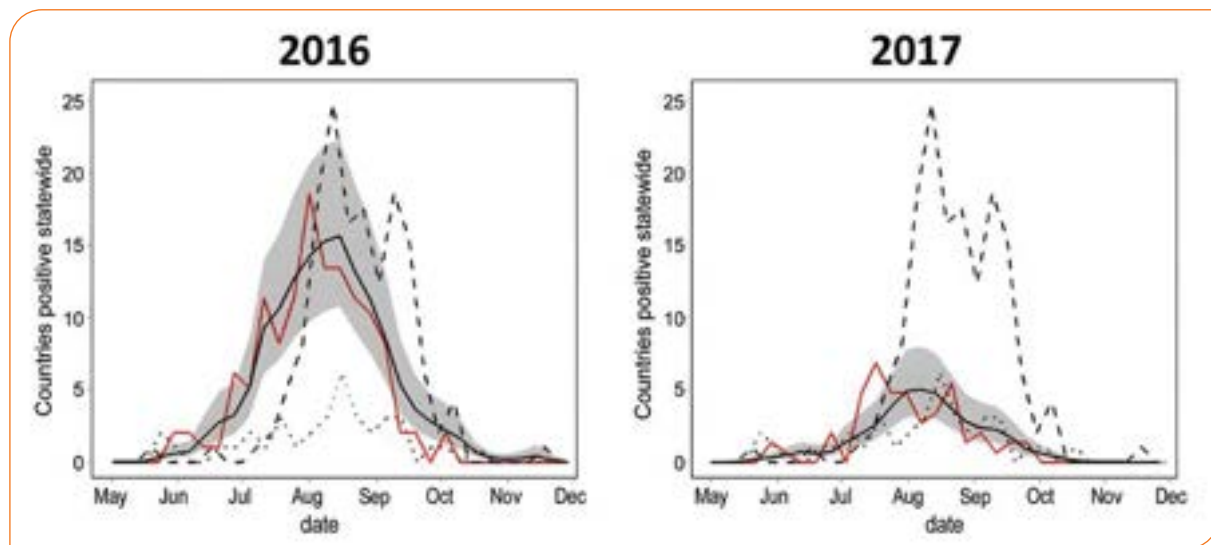
Fig. 4 Prospective WNV forecasts, including the prediction with 95% intervals (black line and gray shading), observed cases in 2016 or 2017 (red line), observed cases (dashed line in 2012, dotted line in 2015) [Attribution: Michael Wimberly, ArboMAP]
