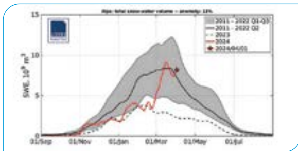
Fig. 5 Total SWE for the Italian Alps, season 2023-24 (red) as opposed to the long-term median (black line) and the 2022-23 season (dashed black line)
