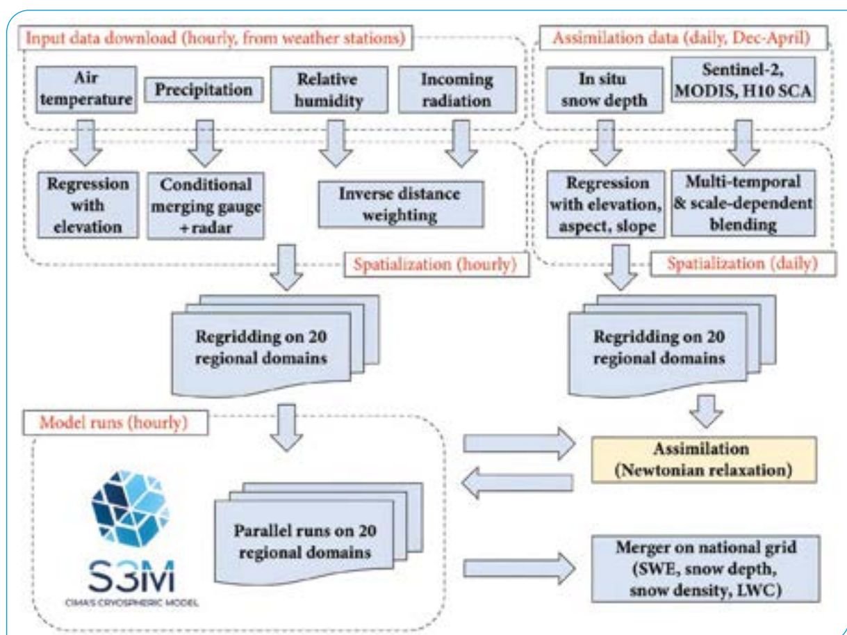
Fig. 4 Schematic of S3M Italy [Attribution: Avanzi et al., 2023: https://essd.copernicus.org/articles/15/639/2023/ ]
