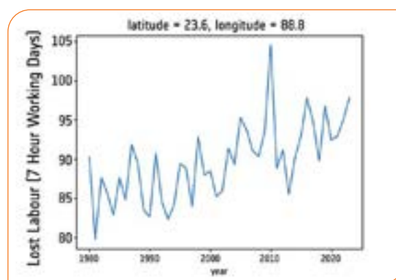
Fig. 1 Total number of working days in which it would have been recommended not to work to remain safe in the heat conditions in Chuadanga district in Bangladesh
