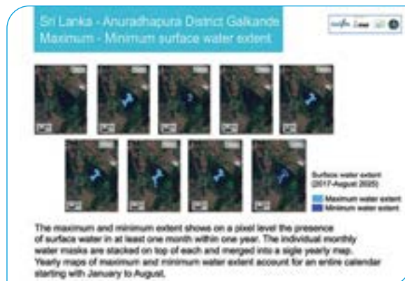
Fig. 6 Minimum and maximum surface water extent over nine years of the Galkande Wewa, District of Anuradhapura, Sri Lanka [Attribution: GeoVille]
