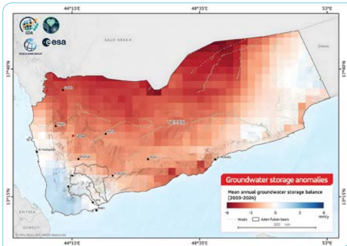
Fig. 2 Mean annual groundwater storage balance (2003–2024) (Attribution: GMV, ESA's GDA water resources)
